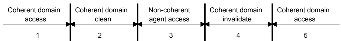
Figure A10.3: Required sequence of communication between coherent and non-coherent domains
